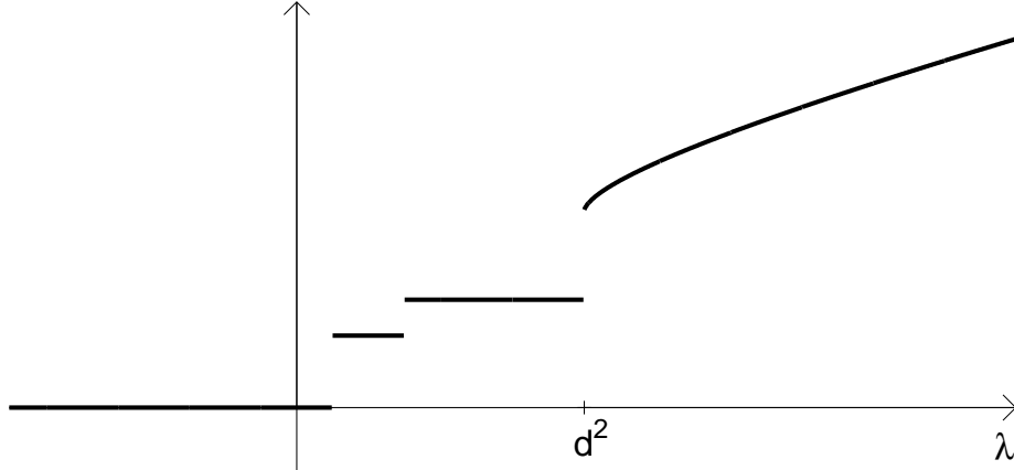
The function \chi_m(\lambda) .
